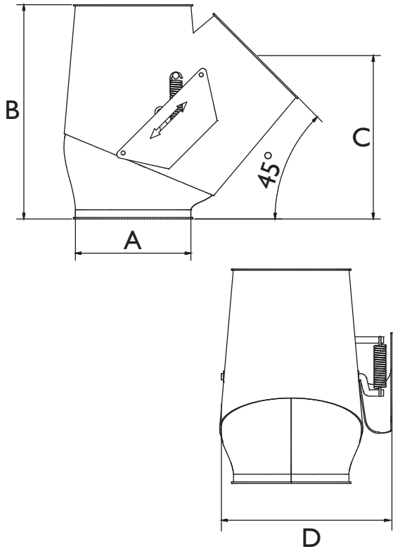
offset-valve 1 x 45°
